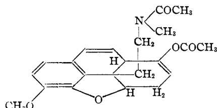
VIII. Des-N-acetyldihydropseudocodeinone enol acetate
